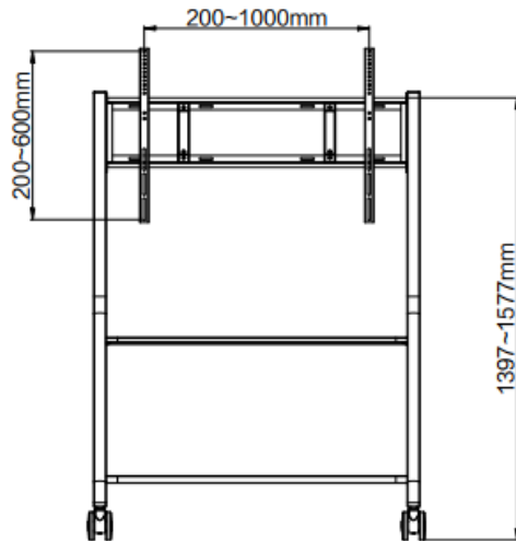
Vista Frontal
